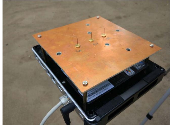
Fig. 9. The WiFi receiver with the hand-made antenna system.
